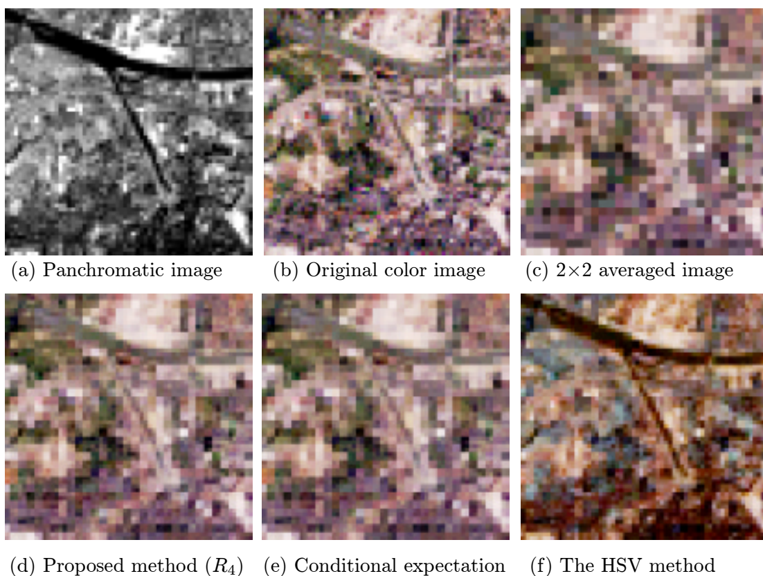
Figure 6: Data fusion of the panchromatic image (a) of size 120 \times 120 and the low-resolution colored image (c) of size 60 \times 60 . (c) is derived by 2 \times 2 averaging procedure of the target 120 \times 120 image (b). (d): correction by the proposed method with g = 5 , r = \sqrt{8} , \beta = 0.8 , (e): correction by the conditional expectation, (f): correction by the HSV method. Images (a) and (c) are LANDSAT 7 images courtesy ESA 1999 – distribution Eurimage, Hasselt, Belgium.
